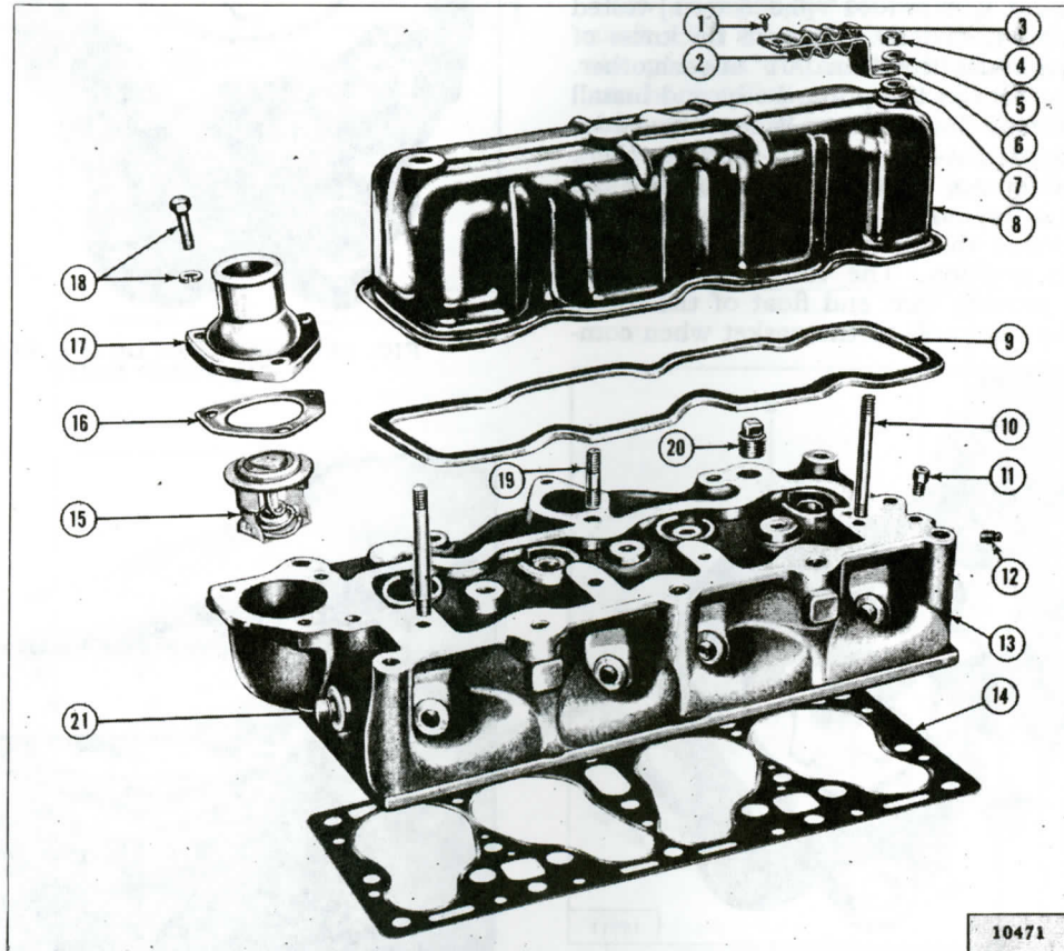
FIG. 100—CYLINDER HEAD
